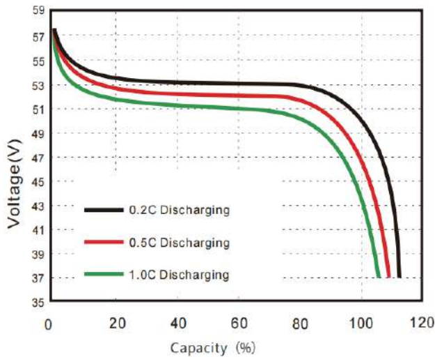
● Different Rate Discharge Curve @25°C
